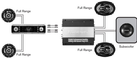
3 Channel Combo (2ch HP + 1ch Subwoofer)
