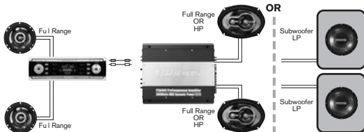
2 Channel (Full-Range, HP, LP)
