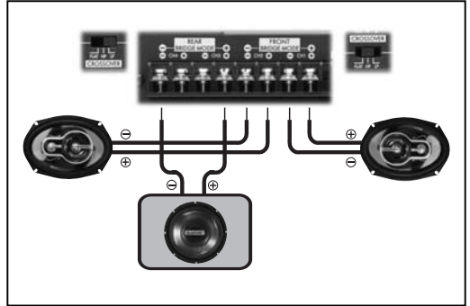
3 Channel Combo (2ch HP + 1ch Subwoofer)
